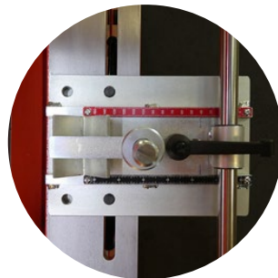
Front roller Vee brackets with new positioning scales
